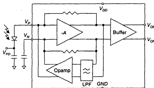
Fig. 2. Block diagram of the fully differential TIA.
