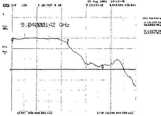
Fig. 3. Relative optoelectronic response of the photodetector and the TIA combination, indicating a 3-dB optical bandwidth in excess of 9 GHz.
